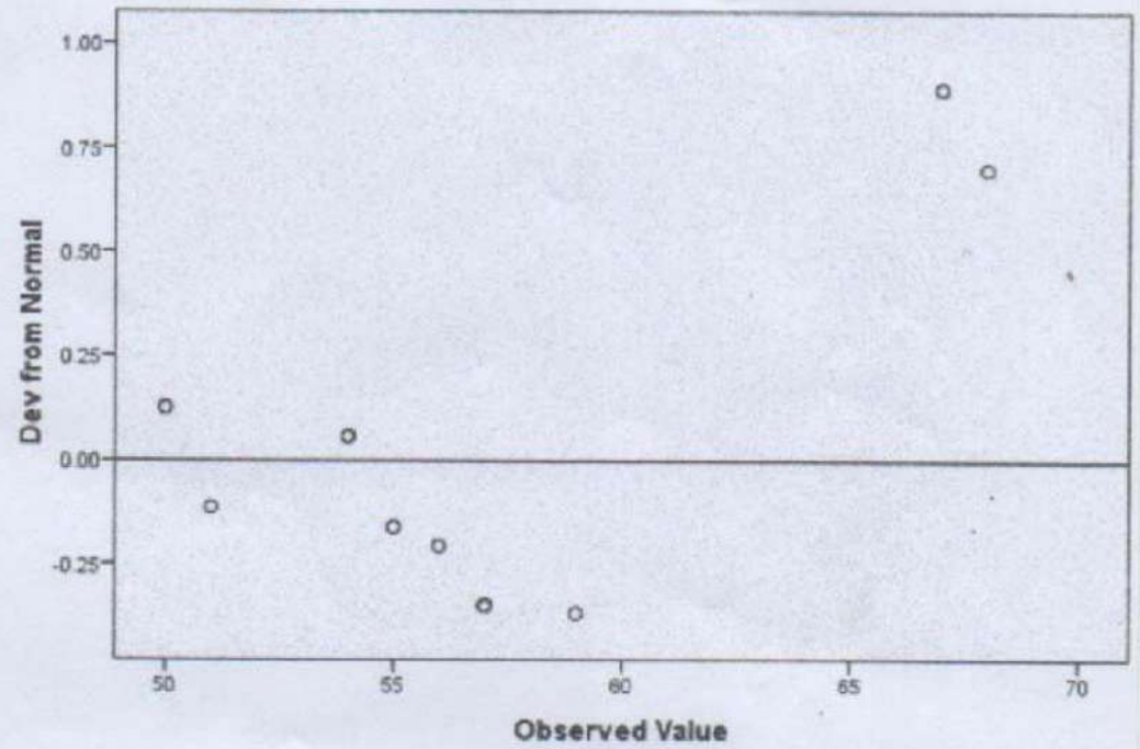
Detrended Normal Q-Q Plot of sesudah
