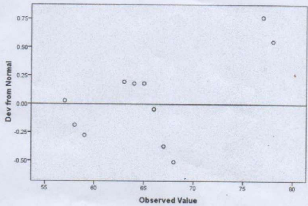
Detrended Normal Q-Q Plot of sebelum
