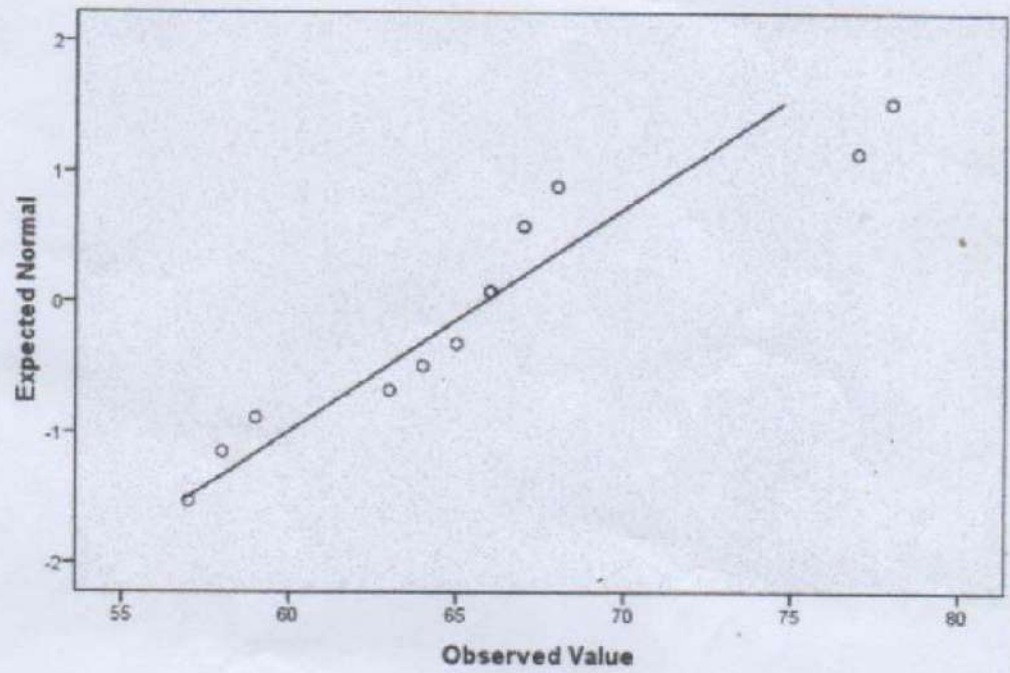
Normal Q-Q Plot of sebelum
