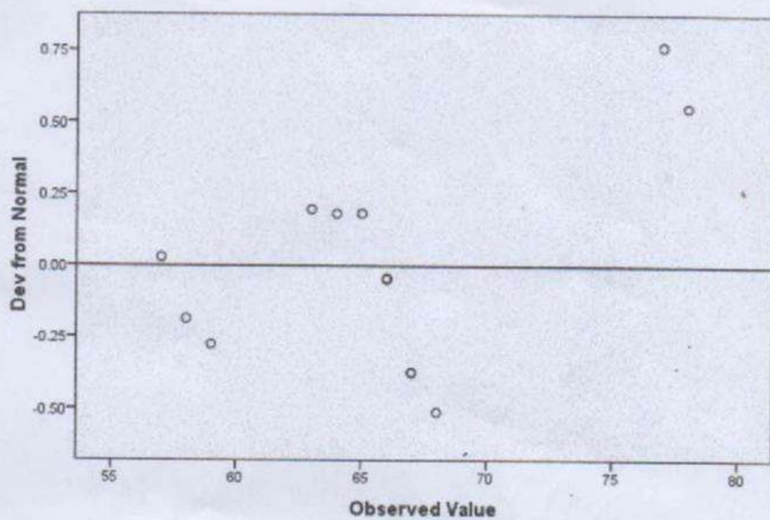
Detrended Normal Q-Q Plot of sebelum
