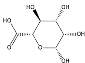
Mannuronic acid
