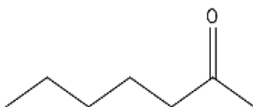
2-Heptanone
