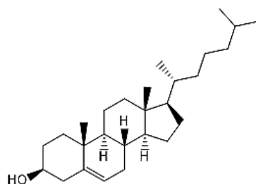
Cholesterol
