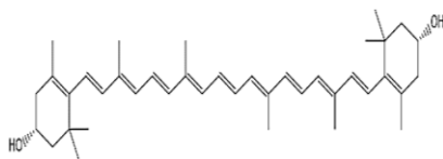
Zeaxanthin
