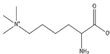
Laminine
