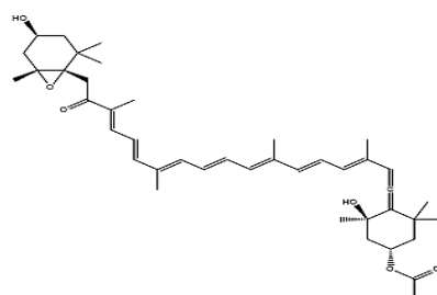
Fucoxanthin
