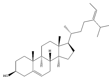
Fucosterol
