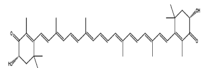
Astaxanthin
