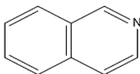
Isoquinoline
