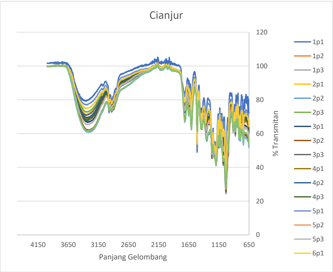
Lampiran 8. Spektrum FTIR Cianjur
