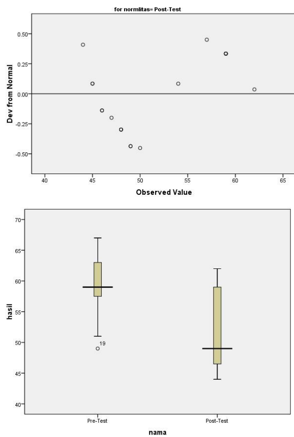
Detrended Normal Q-Q Plot of hasil
